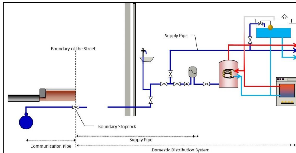
Diagram of Communication pipe and Supply pipes
